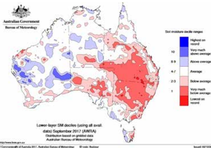
Figure 2 Lower level soil moisture is well below average for much of eastern Australia and South Australia
