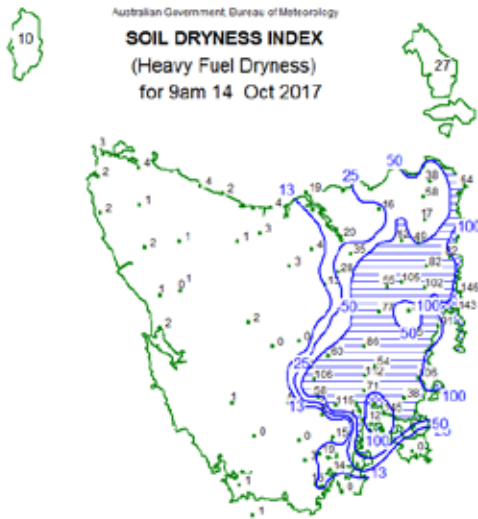
Figure 1 Soil conditions are already extremely dry across eastern Tasmania. These conditions are normally prevalent in late summer!
