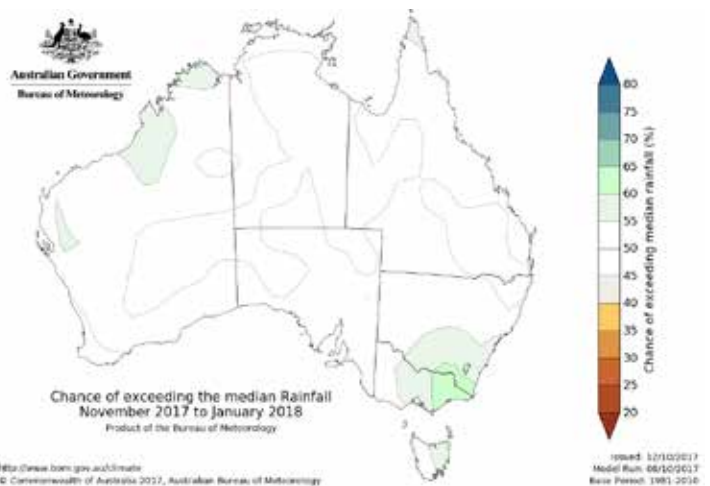
Figure 4 There is a small chance that we may have above average rainfall this early summer.
