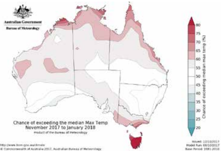
Figure 3 Tasmania will experience a hotter early summer (hotter than on average).
